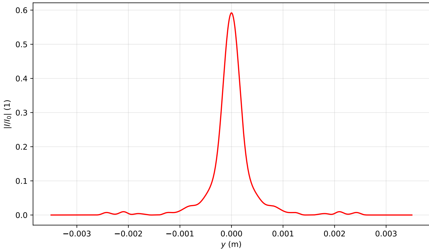
Intensity profile I(x=0, y, z=2.707)/I_0 , P_{in}=4.0P_{cr} , artificial time
